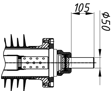
Pic.2 Screw connector (supplied optionally)
