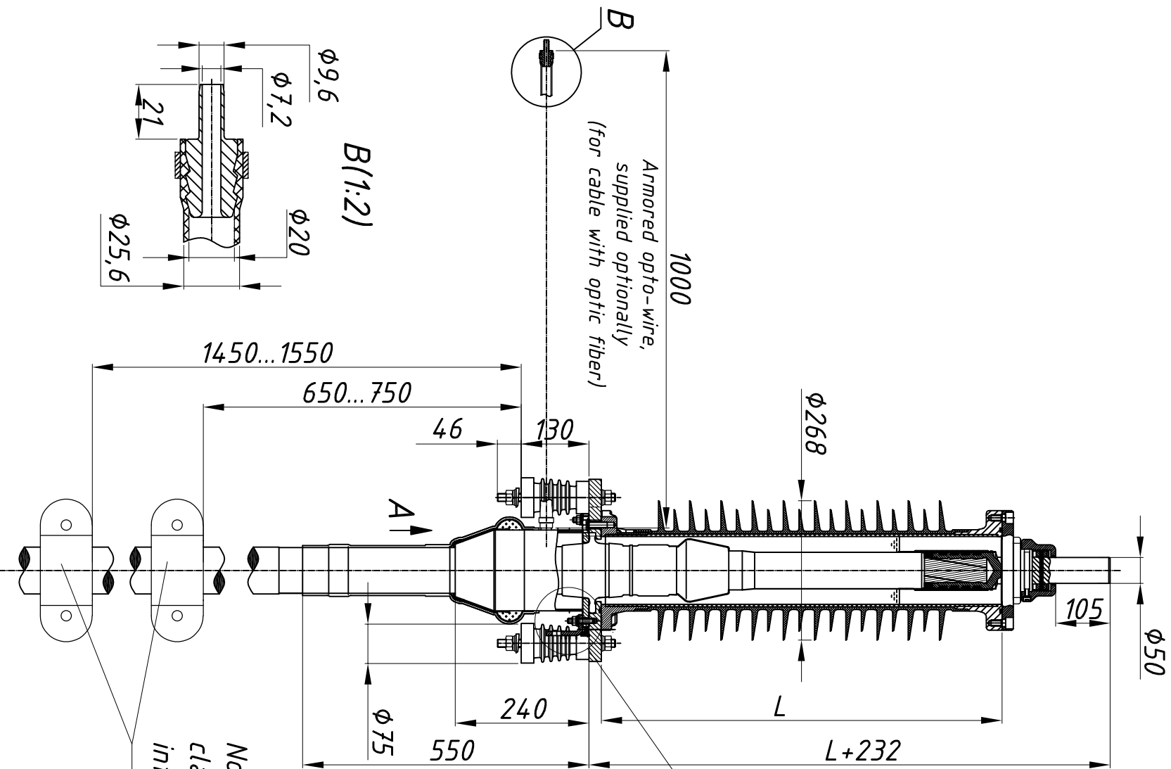
Pic.1 Crimp connector
