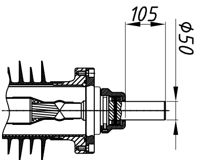
Pic.3 Welded connector (supplied optionally)
